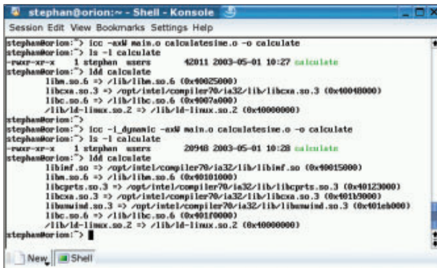
Figure 2: After compiling, a call to ldd shows the libraries that the program will load dynamically. Statically linked libraries are not displayed
