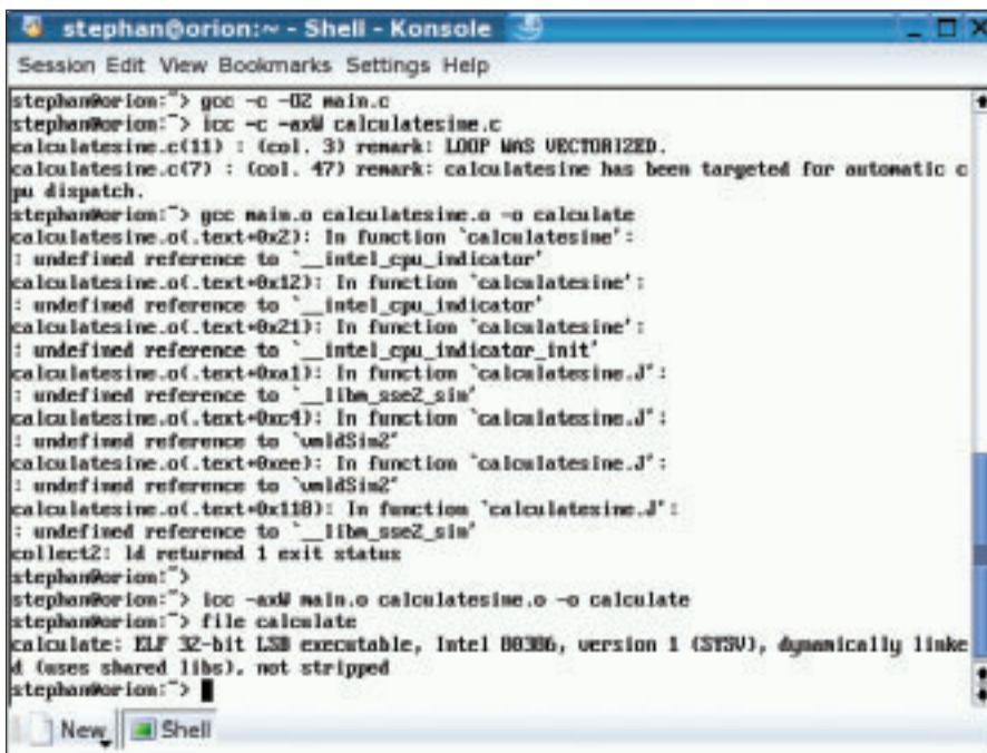
Figure 3: The Intel compiler uses the optimized Libimf library for mathematical operations. To link the results using gcc , the libraries need to be specifically included
