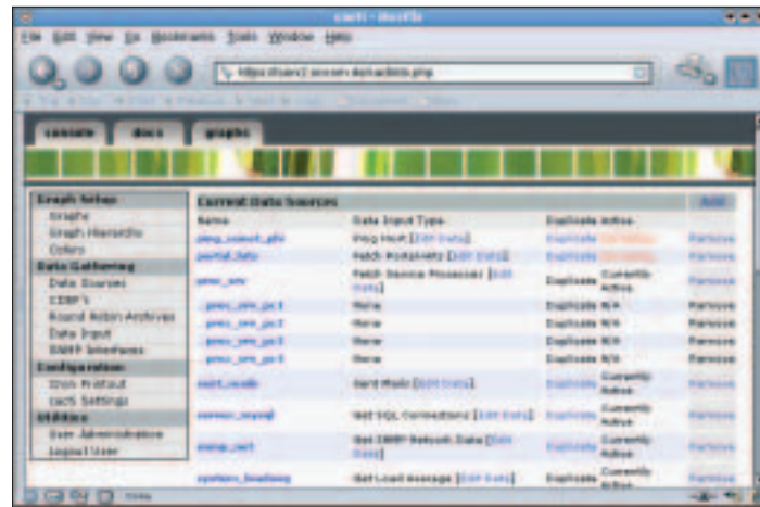
Figure 3: The Current Data Sources table lists the configured data sources. Cacti automatically generates sub-entries for scripts with multiple return values
